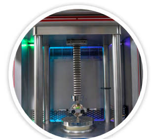
Rigid load frame for minimal machine vibration
